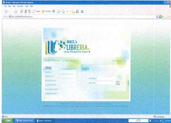
Login Screen
