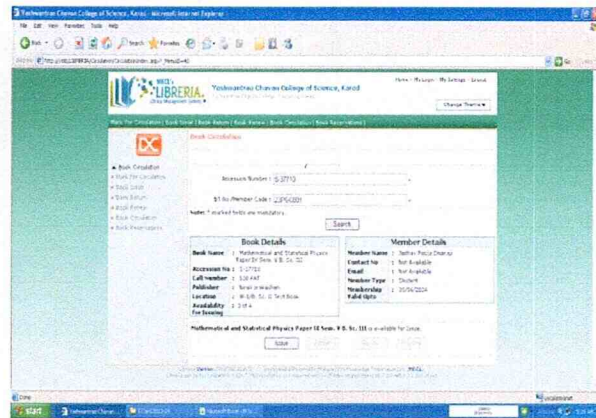
Circulation Screen
